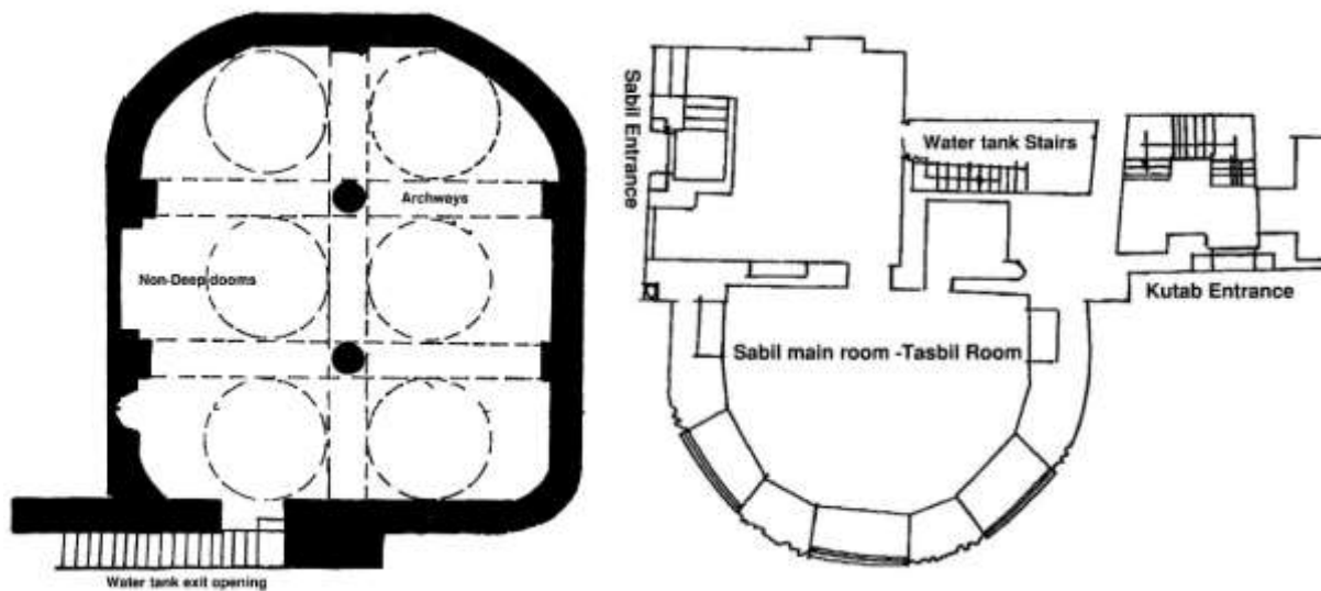
Figure 3: to the left Water tank of Sabil Sultan Mahmoud located in Habbaniyah- Cairo, the right plan is for the first floor, Sabil main room (Tasbil room) [17].
